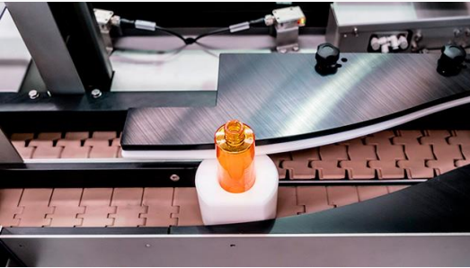
Puck Introduction for unstable or delicate bottles for easy line set-up
